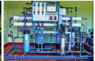
Construction of Nikawewa and Bodagama Water Supply Scheme 10m 3 /day Capacity Reverse Osmosis Plant
