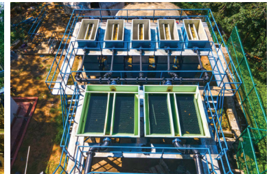
Construction of Bulathkohupitiya Integrated Rural Water Supply Scheme 1000m 3 /day Package Treatment Plant
